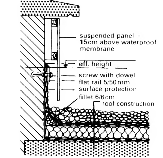
21 Chimney connection with suspended fascia panel
